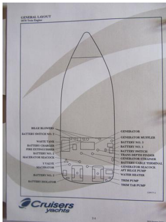
Cruiser 28' Twin engine layout
