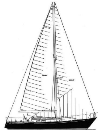
35' C&C Designer Profile Drawing
