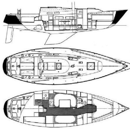
35' C&C Designer Floorplan Drawing
